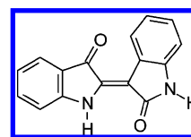
Figure 1. Structure of natural indirubin.
